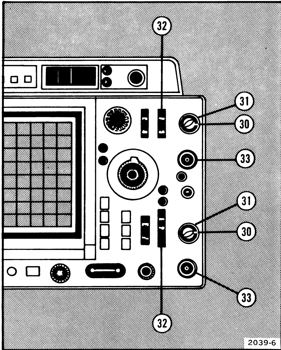
Fig. 5. Trigger controls, connectors, and indicators.
