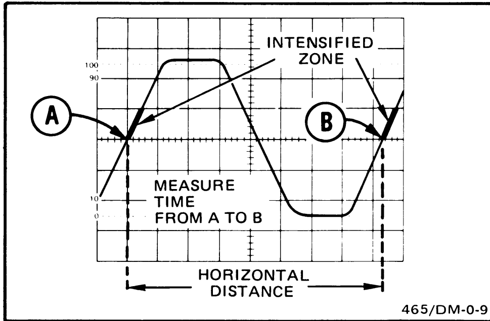
Fig. 26. Time duration.
