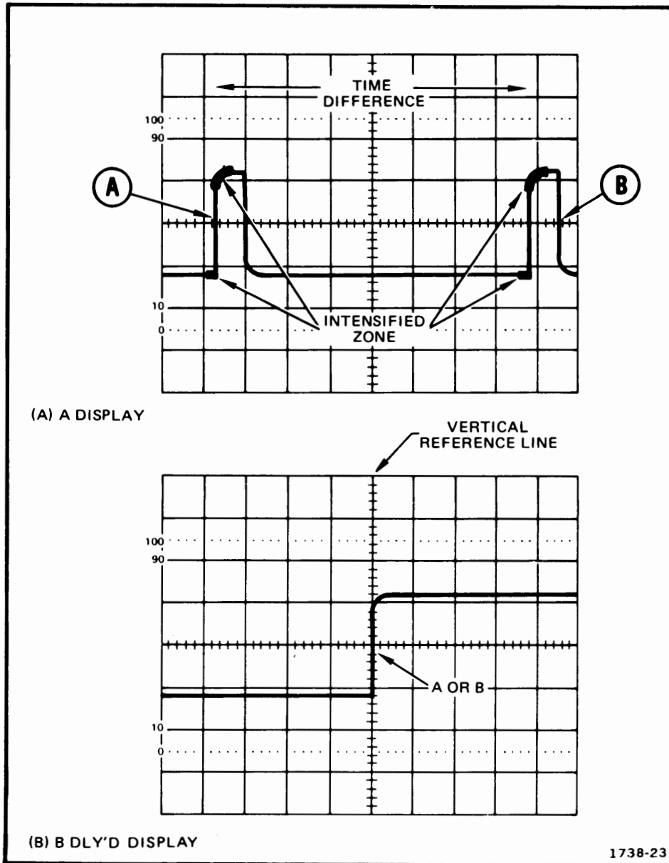
Fig. 25. Time difference between repetitive pulses.
