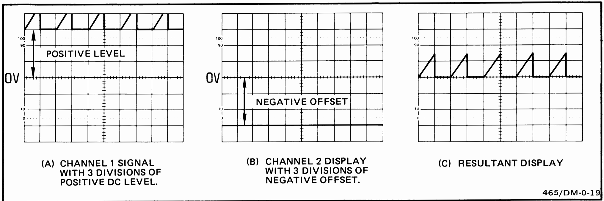
Fig. 16. Algebraic addition.
