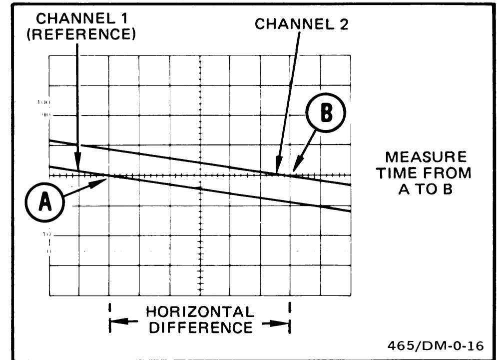
Fig. 22. High-resolution phase difference.
