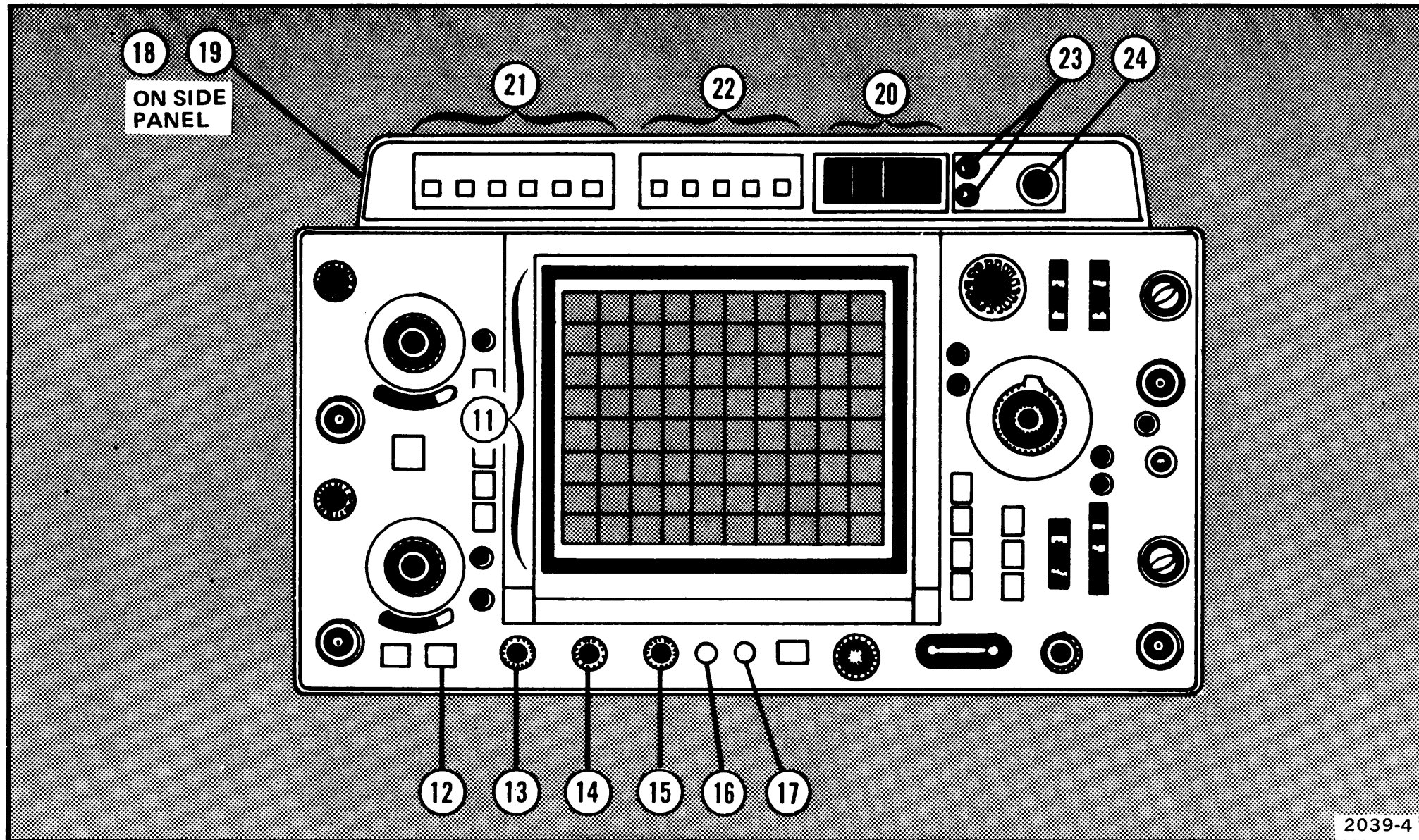
Fig. 3. Display and DM44 controls, connectors, and indicators.
