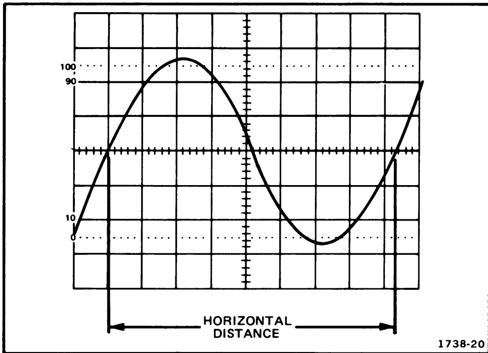
Fig. 18. Time duration.
