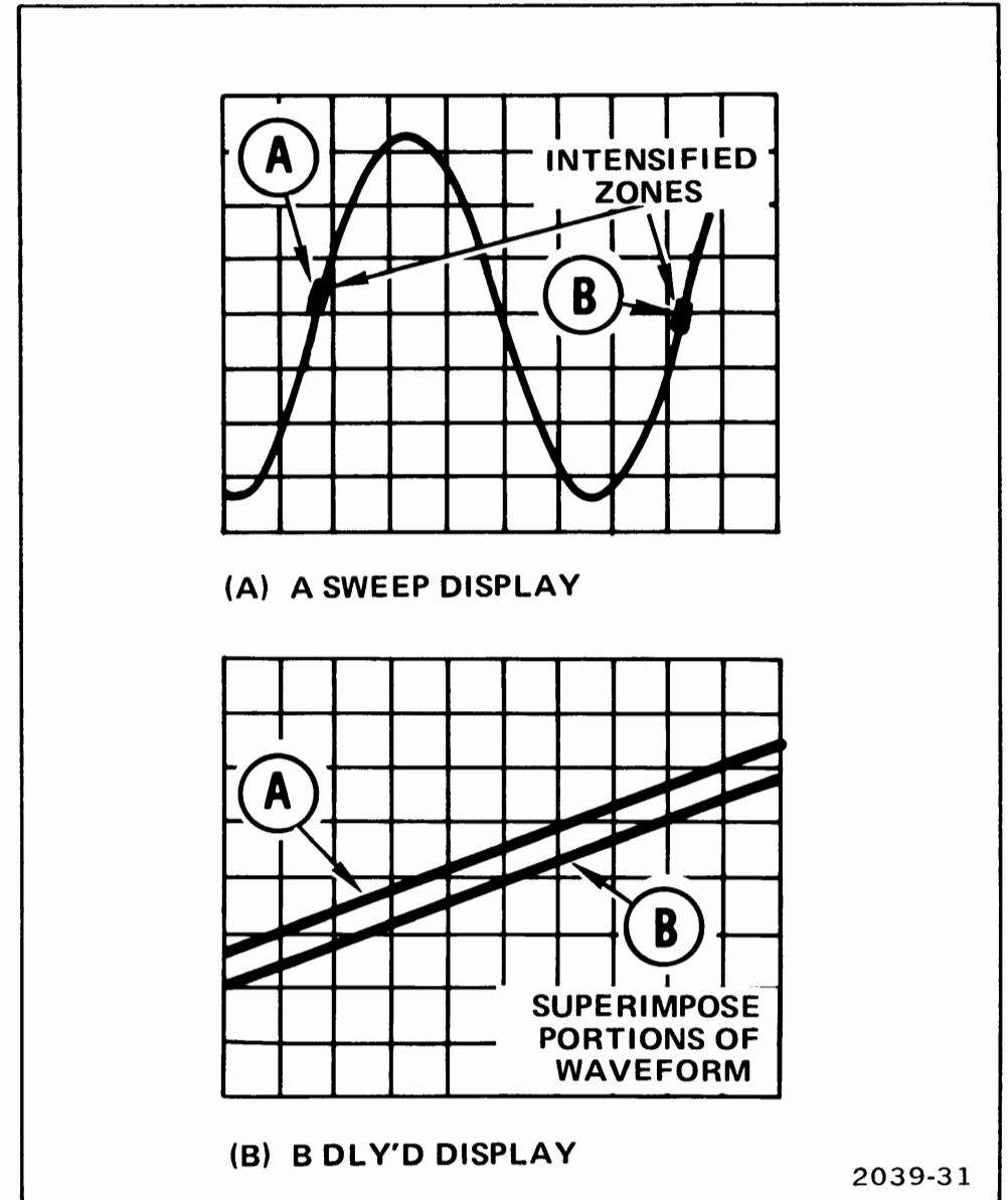
Fig. 30. Time duration and frequency measurements.
