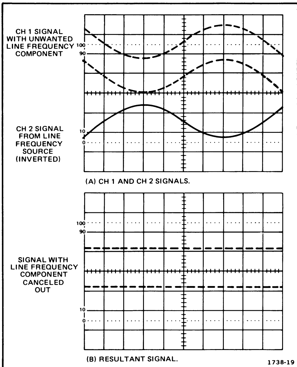
Fig. 17. Common-mode rejection.
