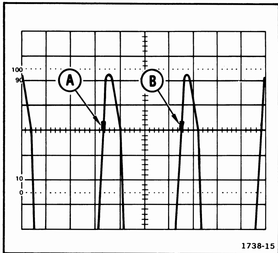
Fig. 13. DM44 timing check.
