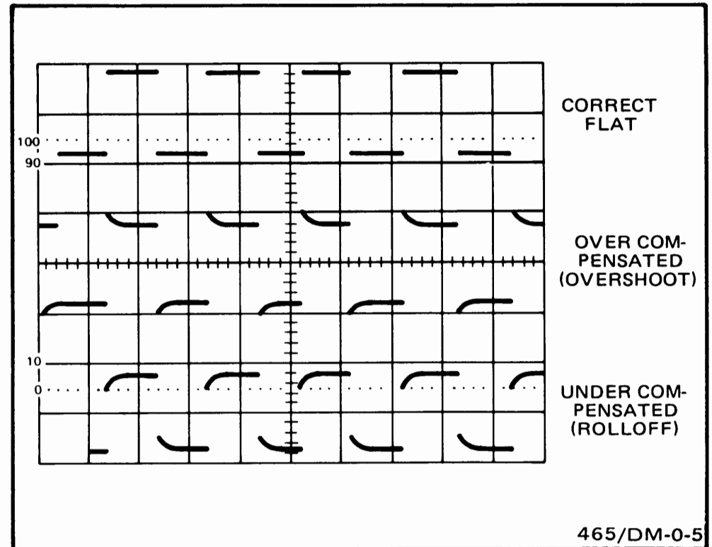
Fig. 11. Probe compensation.
