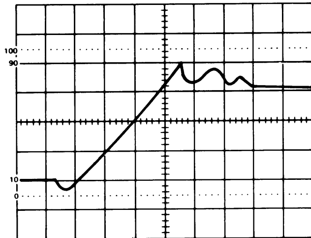
(B) B DELAYED DISPLAY
