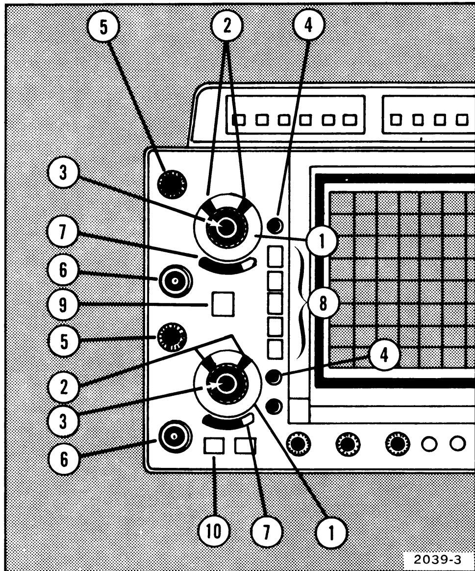
Fig. 2. Vertical controls, connectors, and indicators.
