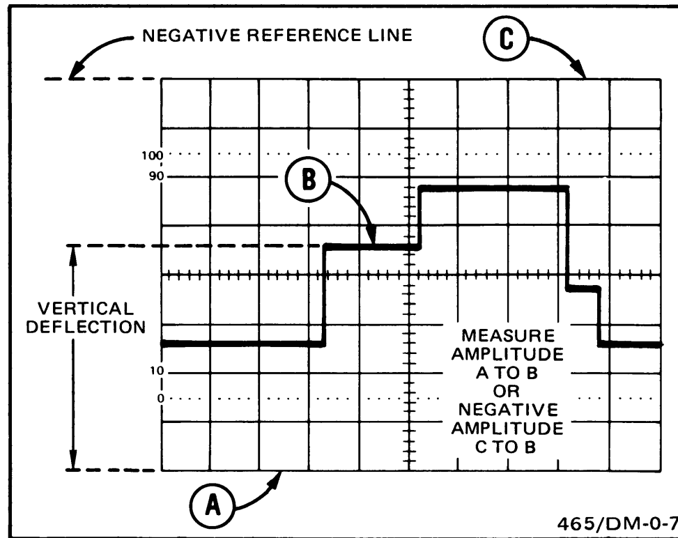
Fig. 15. Instantaneous voltage measurement.
