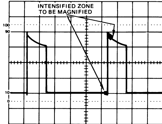
(A) A INTENSIFIED DISPLAY
