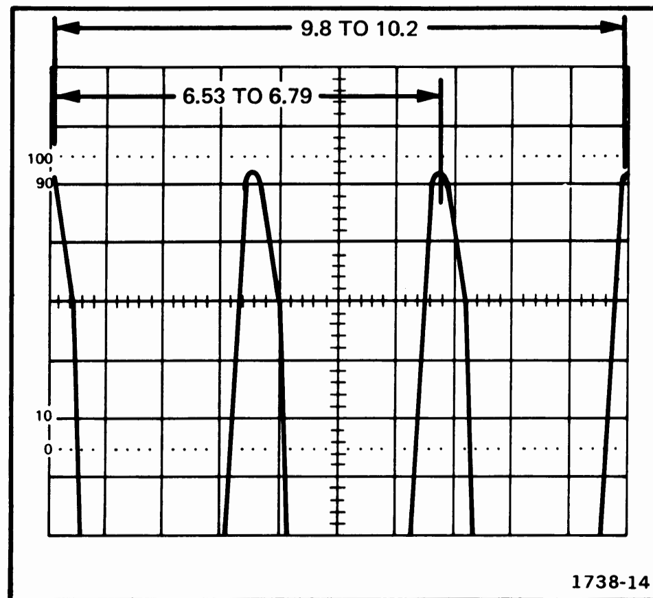
Fig. 12. Basic 465 timing check.
