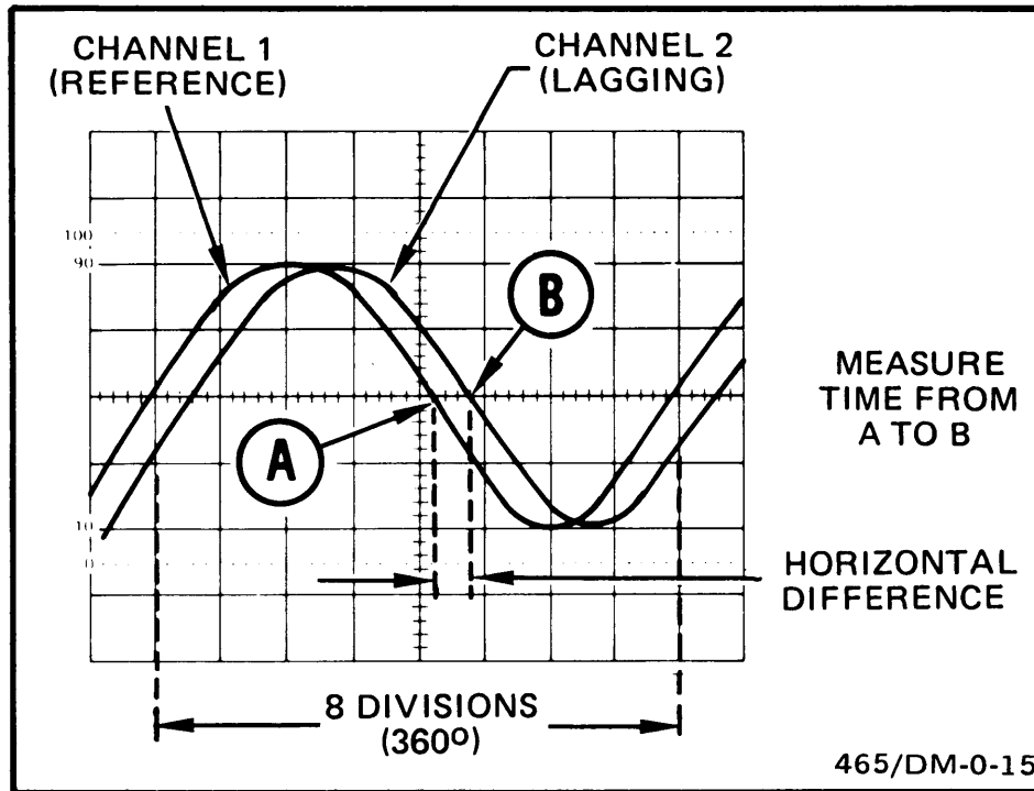
Fig. 21. Phase difference.
