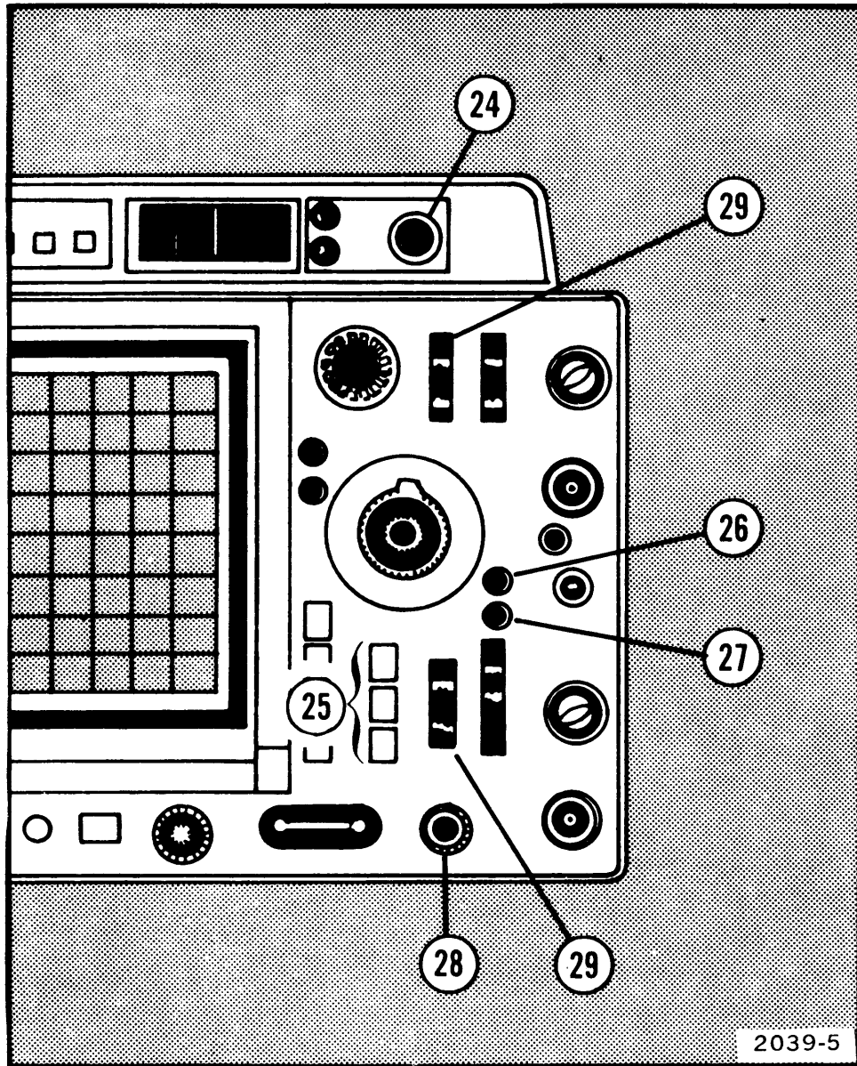
Fig. 4. Trigger controls, connectors, and indicators.
