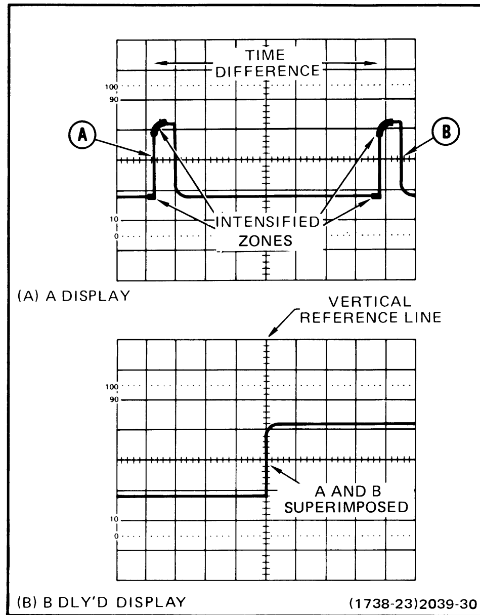
Fig. 29. Time difference between repetitive pulses.
