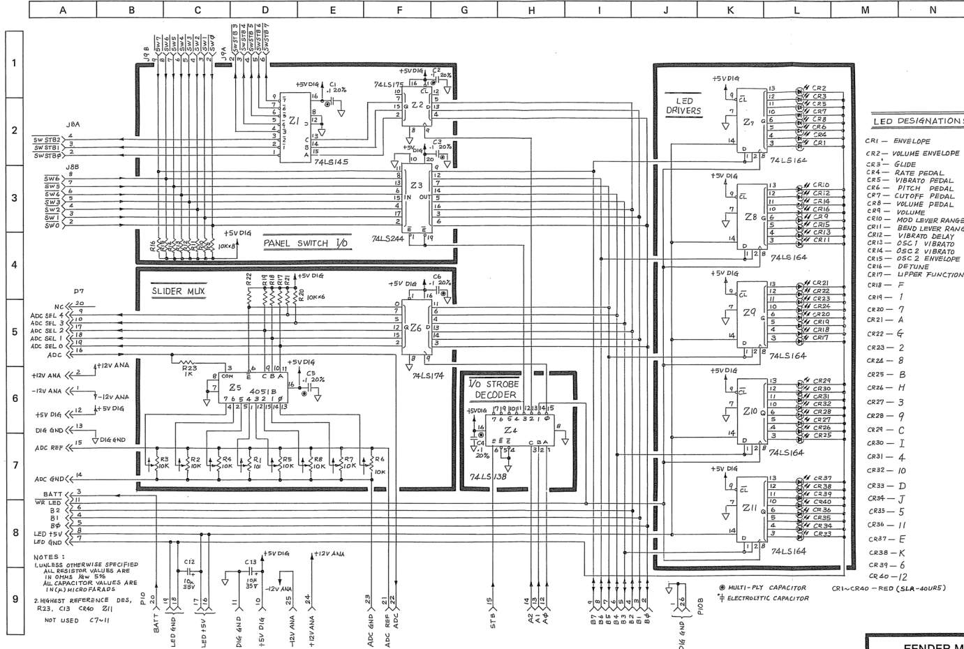
FENDER MI CHROMA POLARIS CONTROL PANEL RIGHT SCHEMATIC
