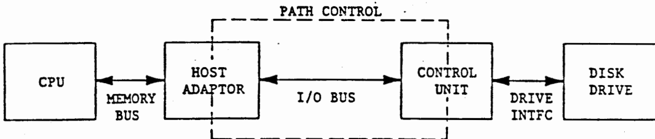
Figure 4-1 : PHYSICAL PATH
