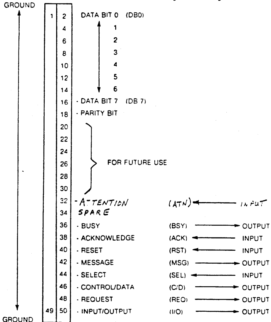
FIGURE 3-1. SCSI Bus Pin Assignments 3-1
