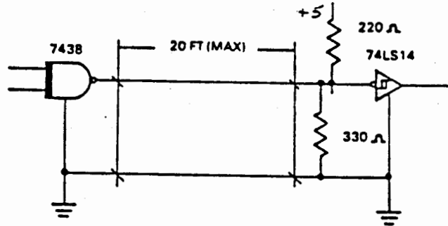
Figure 3-7. Control Driver/Receiver Lines
