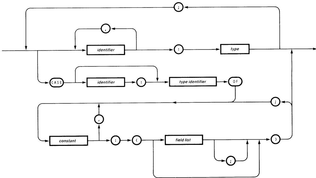
field list
