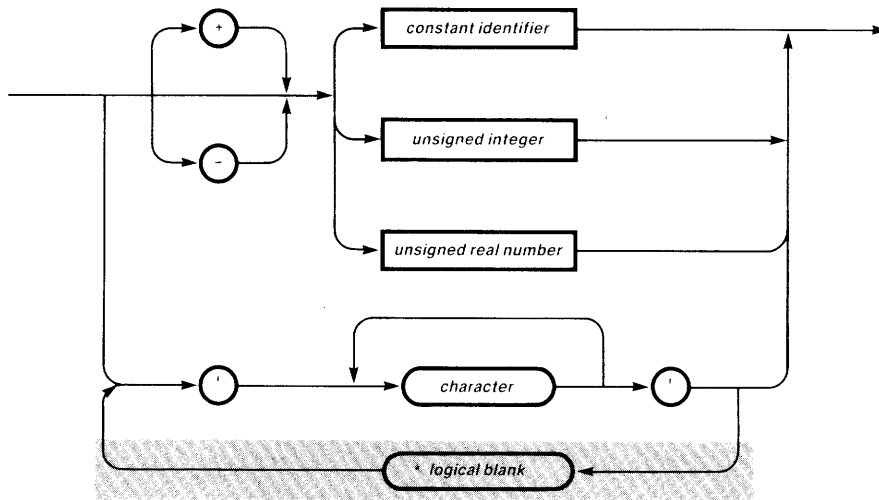
constant
