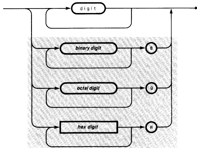
unsigned integer
