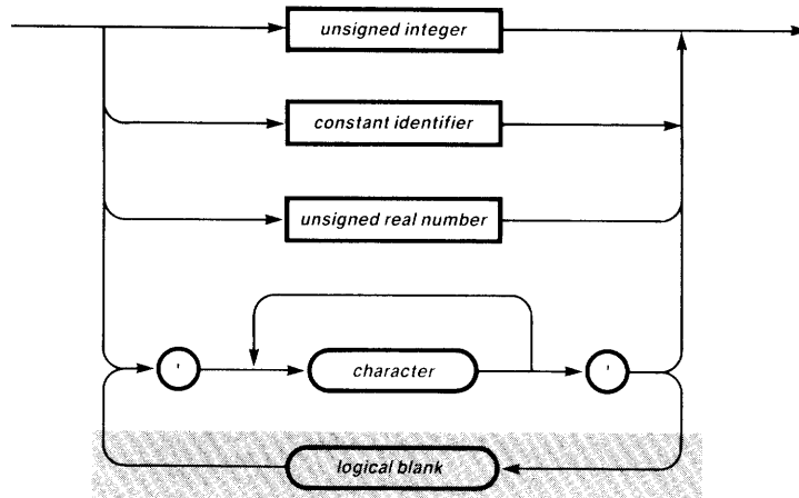
unsigned constant
