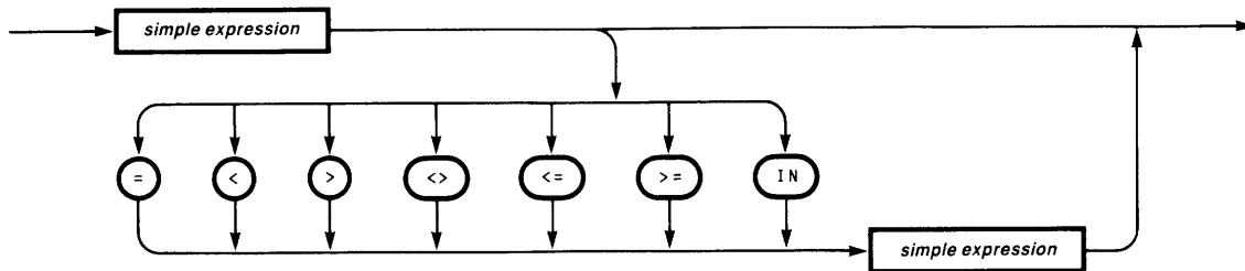
expression
