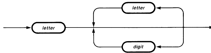
identifier
