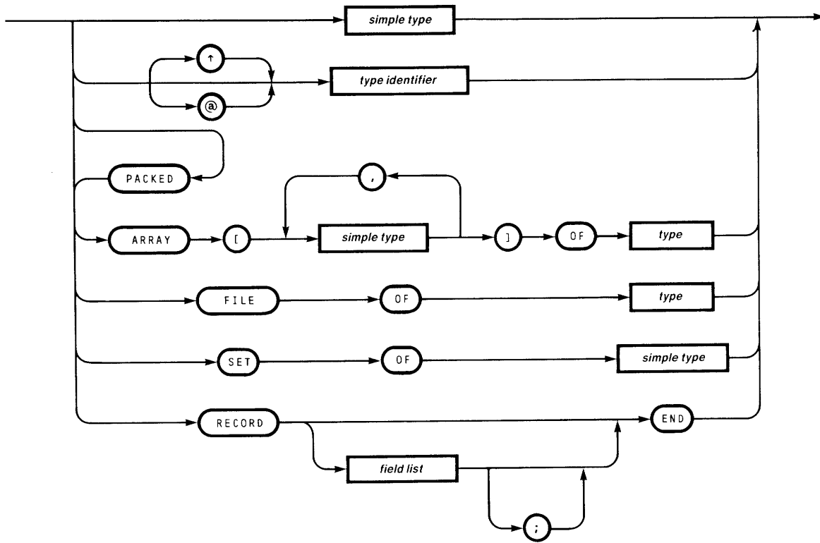
type
