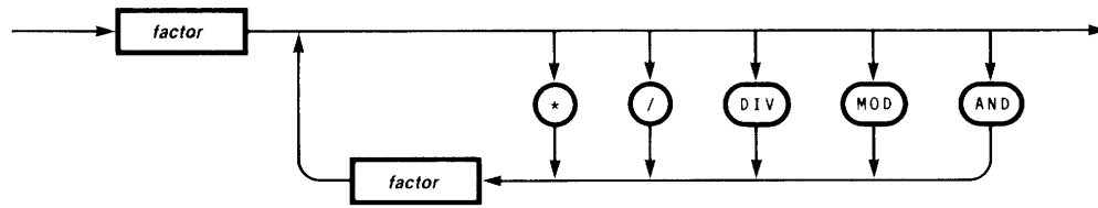
term
