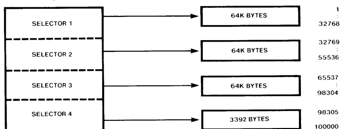
Figure H-3. The Memory Representation of a Large Array Whose Component Size Is a Power of Two
