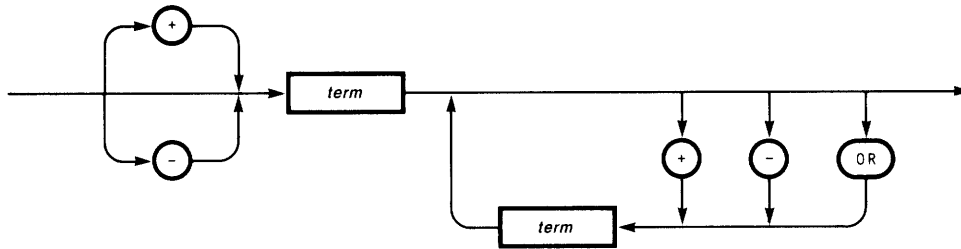
simple expression
