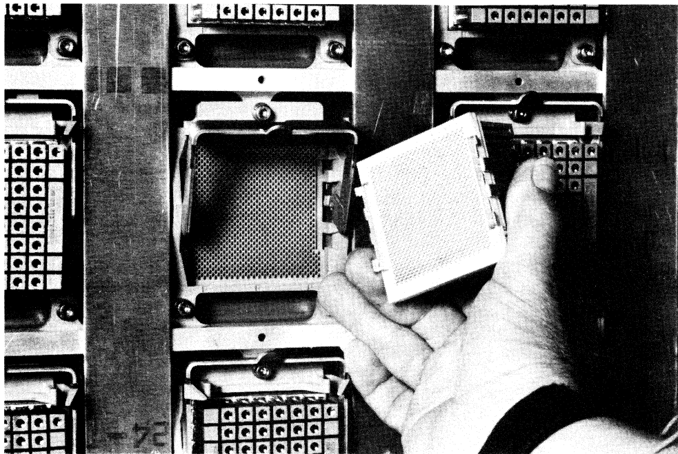
Figure 3. A 64-mm MCM being hand held
