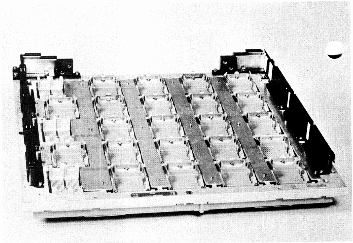
Figure 4. The 4381 MCM board without any modules mounted
