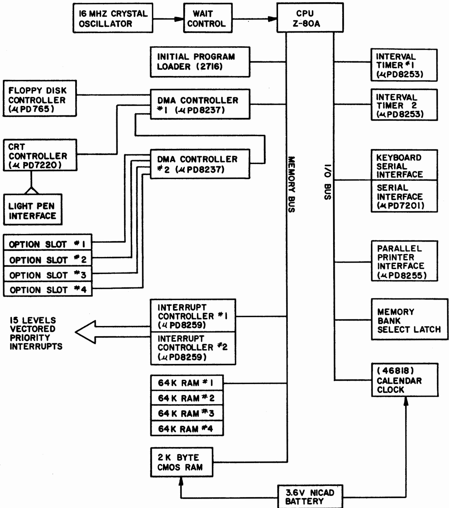
A block diagram of the QX-10 electronics.
