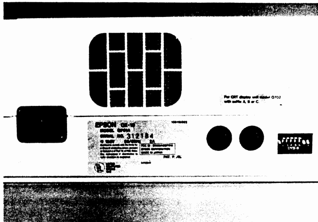
The back apron of the main electronics case showing the power cord connector, the fan, light pen and monitor connectors and the memory configuration DIP switches.
