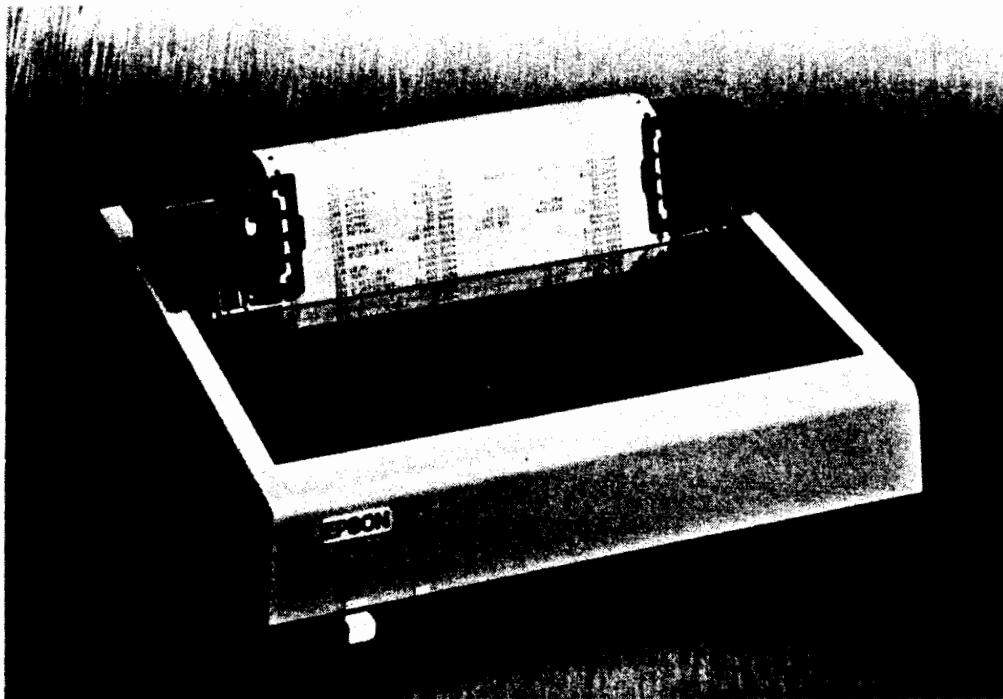
The TX-80 printer, Epson's first dot matrix printer export to the United States. This printer offered a seven dot high matrix (no lower case descenders), a solenoid-operated linefeed mechanism, and could print up to 58 lines per minute. Printing was strictly uni-directional, left to right. Photograph courtesy Epson America Incorporated.
