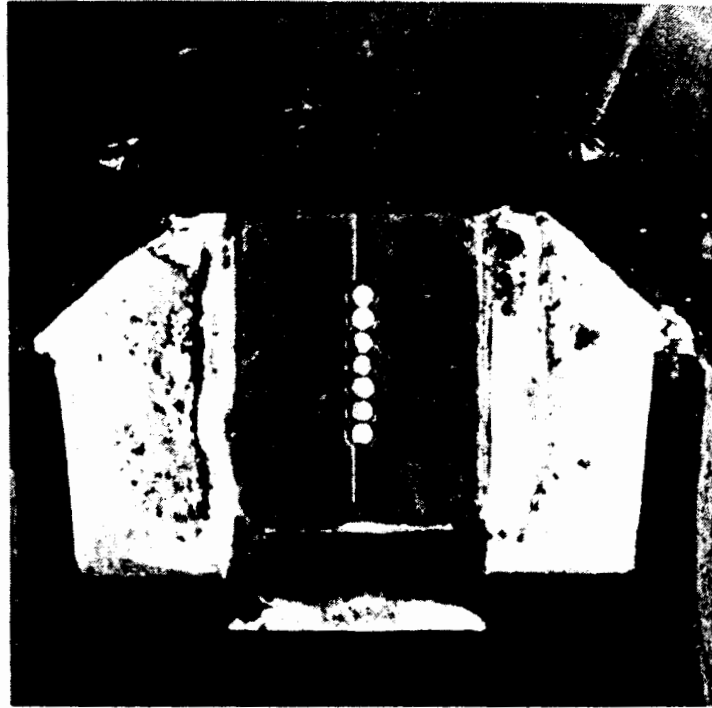
The print wires of a dot matrix printer head. The wires are typically about .012 inches in diameter. This particular head was used in an old Centronics printer.
