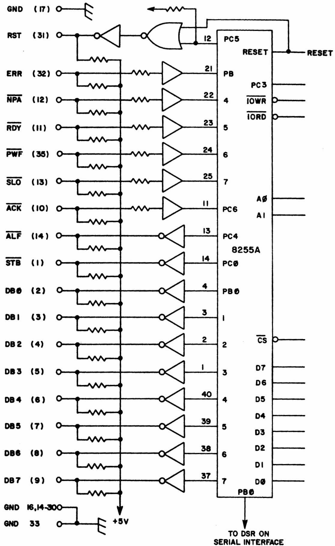
Schematic diagram of Centronics compatible parallel printer interface on the QX-10.
