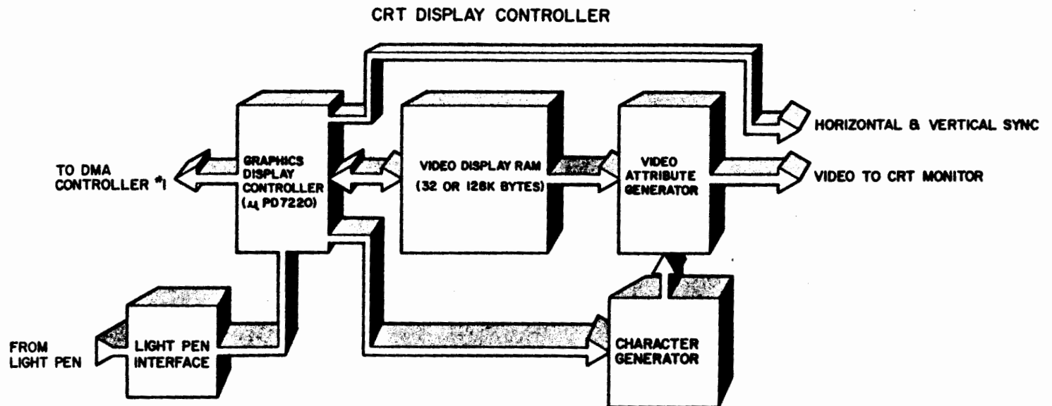
A block diagram of the QX-10 video display controller.
