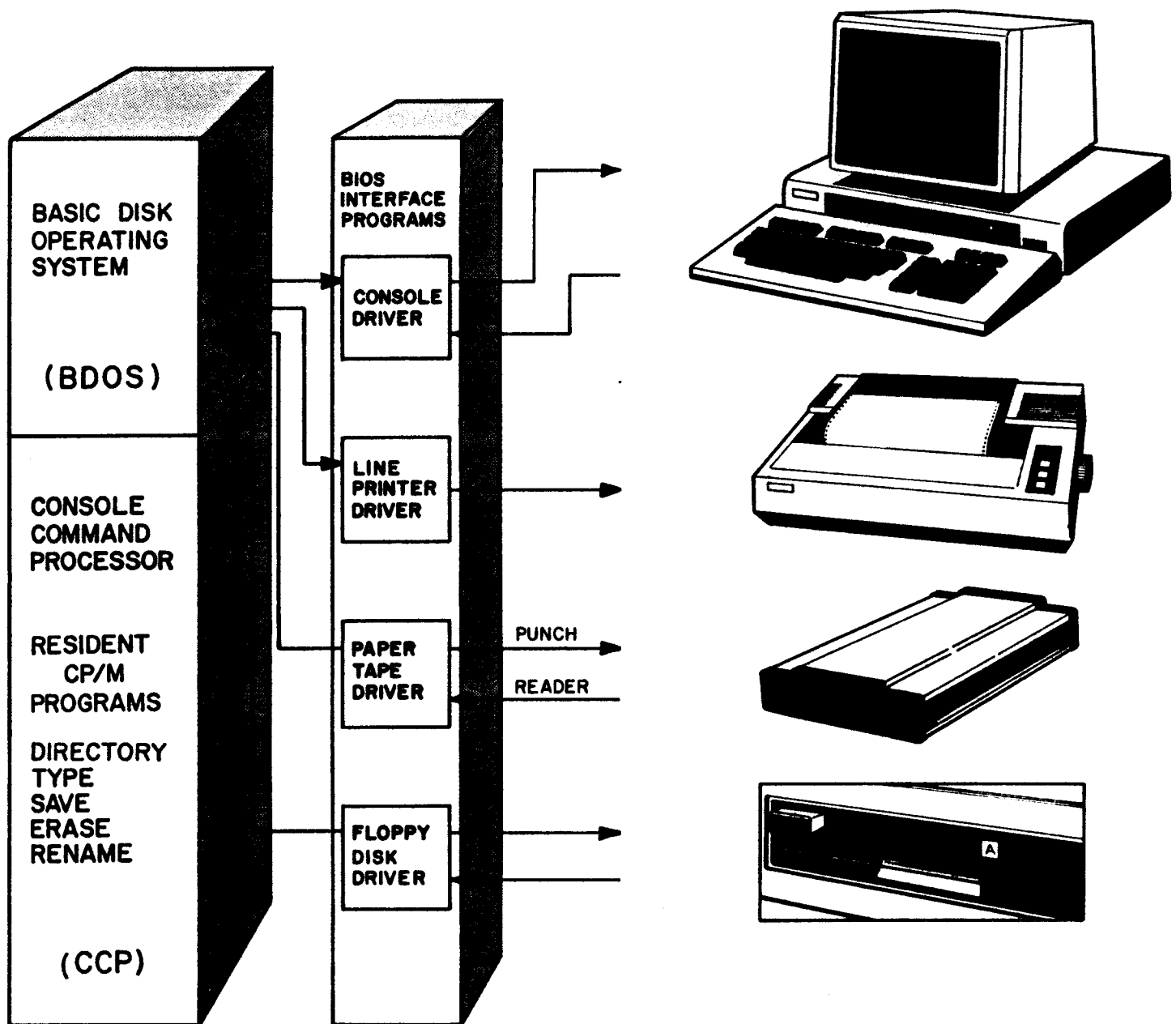
Hardware and software relationships in CP/M operating system.
