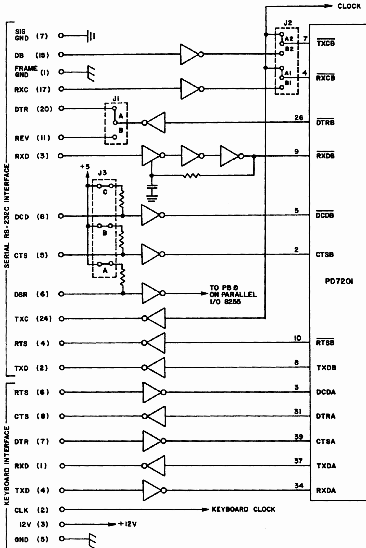
Schematic diagram of serial interfaces used by the QX-10 for the keyboard and RS-232C interface.
