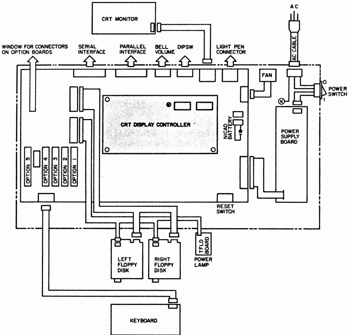
Internal cabling diagram of the QX-10.
