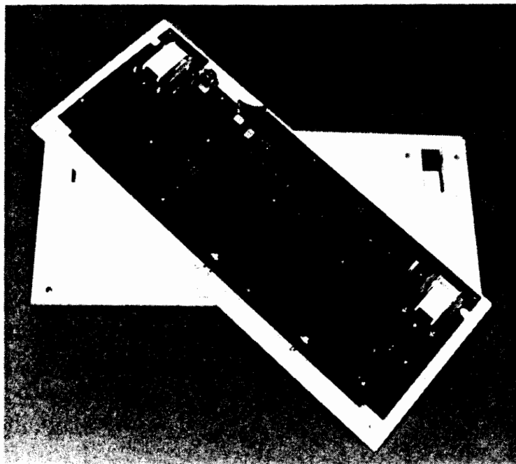
Inside the Brother HASCI keyboard. Notice the legs are attached to the top cover through the printed circuit board, rather than the bottom case.
