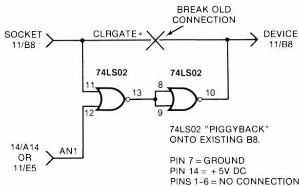
Fig. A-1. Schematic for the Apple IIe color killer modification.
