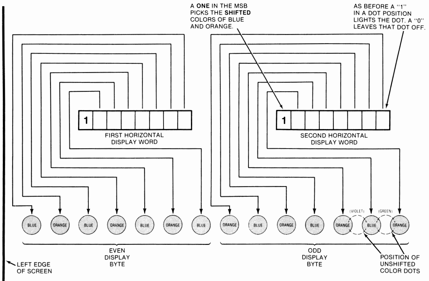
Fig. 8-2. How shifted colors are mapped onto HIRES screen. MSB of each display word shifts or unshifts seven dots at once.
