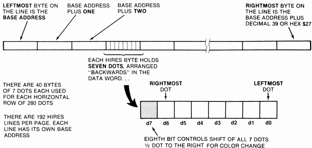
Fig. 7-5. Details of one horizontal line mapping.
