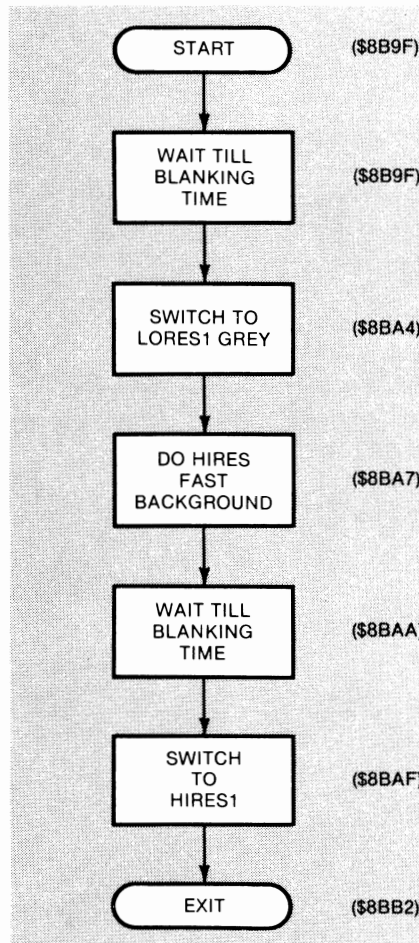
Fig. 8-5. Flowchart of optional "Invisible Switcher."
