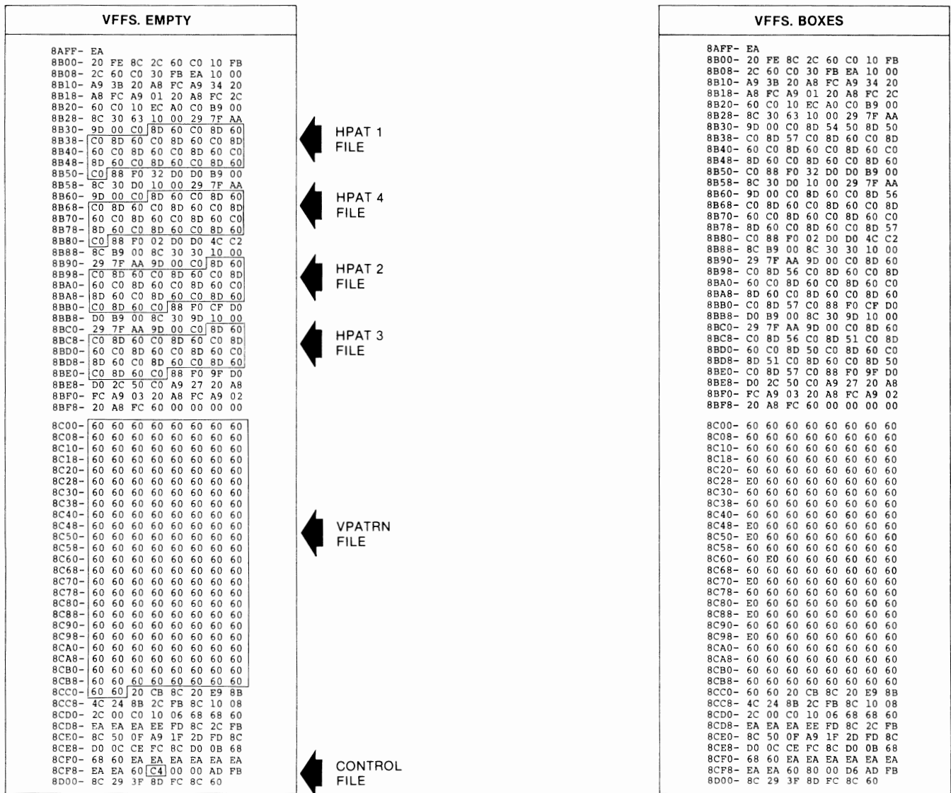
Fig. 5-5. Hex dumps of VFFS files used in
