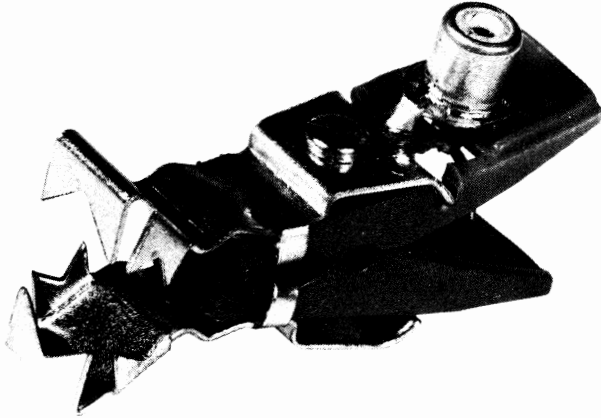
Glomper of the first kind is made from a phono jack and a clothespin connector. Use it if you often change or test different tv's.
