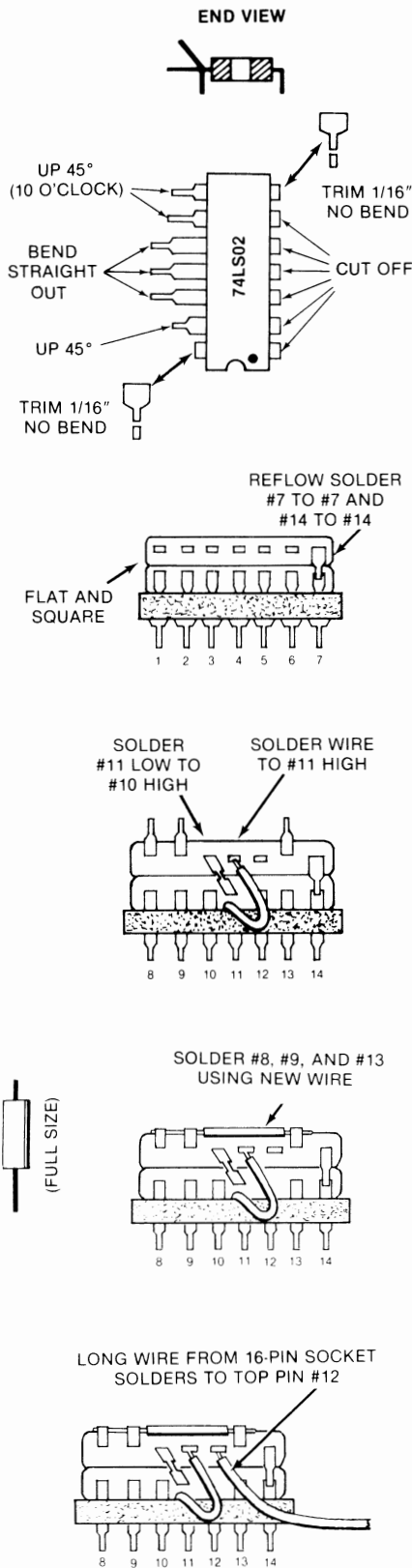
Fig. A-2-cont. How to build the Apple IIe color killer.
