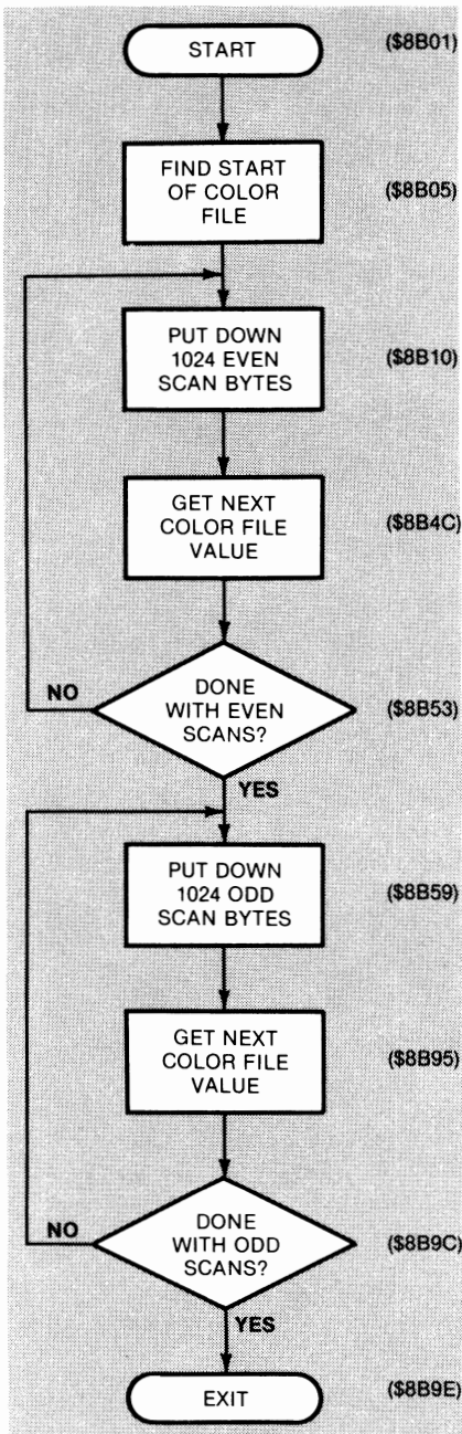
Fig. 8-4. Flowchart of FAST BACKGROUND.SET program.
